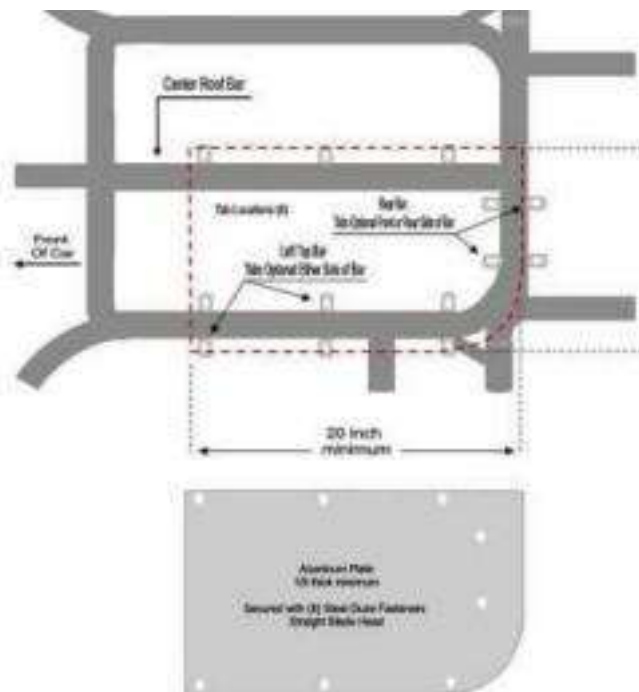
Exhibit 3: Roof Panel Construction
